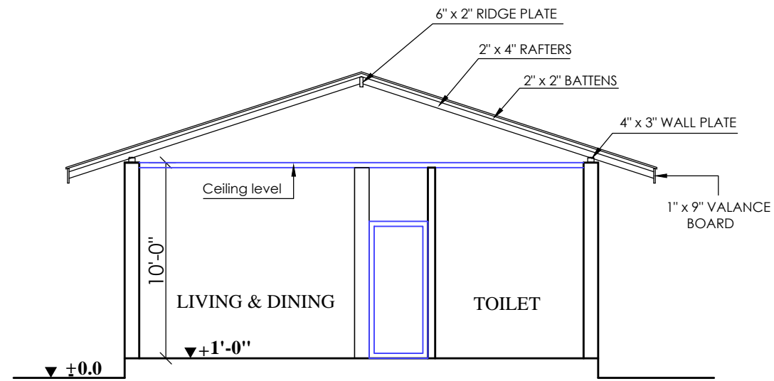
SECTION X-X SCALE - 8 FEET TO AN INCH
