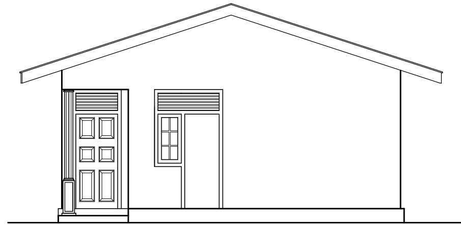
SIDE ELEVATION SCALE - 8 FEET TO AN INCH
