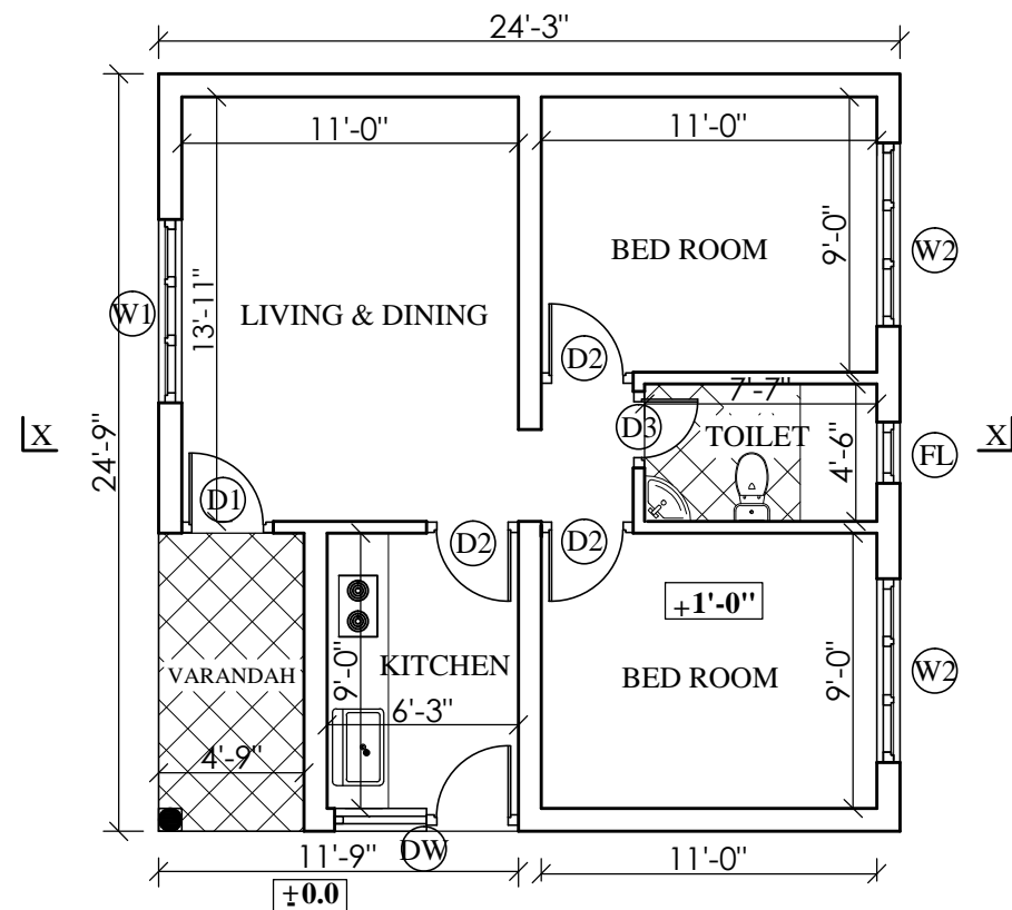
FLOOR PLAN SCALE - 8 FEET TO AN INCH Floor Area - 599.17 Sq.Ft
